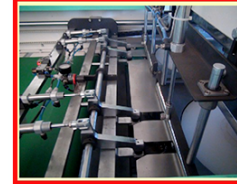
Folding system
